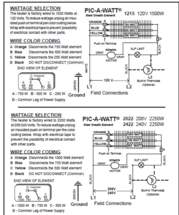
Wiring Diagram Figure 5
